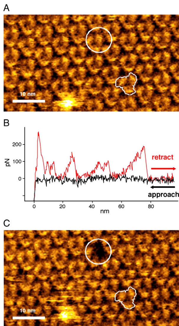
Fig. 8. Mechanical unfolding of single bacteriorhodopsin molecules in purple membrane. (A) Contact mode AFM image of purple membrane before SMFS exhibiting the distinctive trimeric structure of bacteriorhodopsin. (B) F–D curve collected during SMFS representing the mechanical unfolding of a single bacteriorhodopsin molecule (red trace). (C) Contact mode AFM image of purple membrane after collection of the F–D curve revealing the empty space left by the extracted bacteriorhodopsin molecule (highlighted by white circle). Reprinted with permission from [78] and The American Association for the Advancement of Science.
